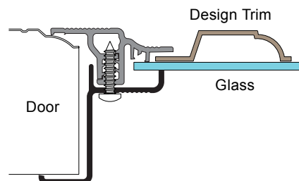
SRF- SG Style Window Frame
