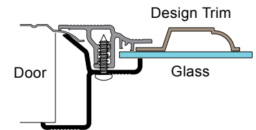
SRF- IP Style Window Frame
