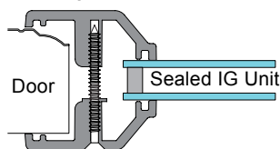
CMF- IG Style Window Frame
