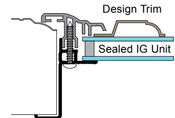
AWF-CLASSIC-IG Style Window Frame
