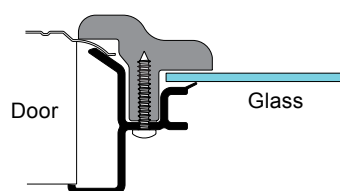
CWF- IP Style Window Frame
