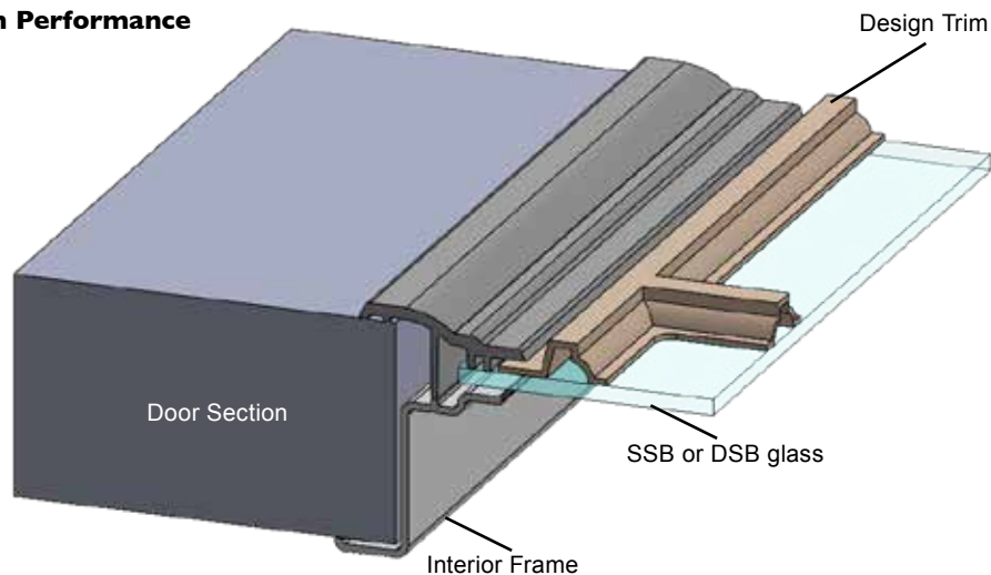
IMF- P Style Window Frame
