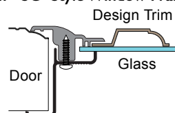
IMF- SG Style Window Frame
