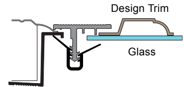
SPWF-PIF Style Window Frame
