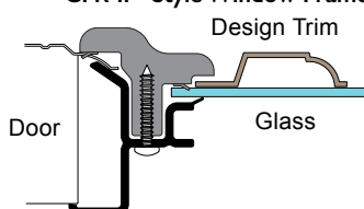
CFR-IP Style Window Frame
