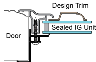
HWF- IG Style Window Frame
