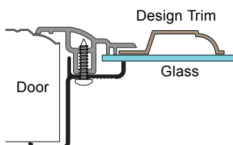
HRF- SG Style Window Frame
