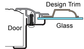
HRF- SG Style Window Frame
