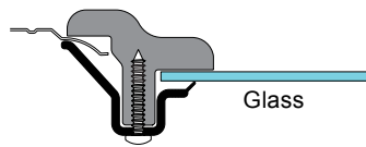
CWF- P Style Window Frame
