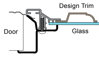
AWF-CONTEMPO-IP Style Window Frame
