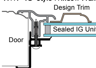
HWF- IG Style Window Frame
