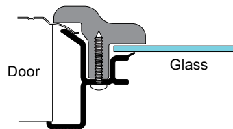
CWF- IP Style Window Frame
