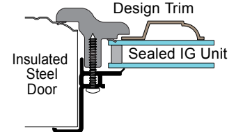
SWF- IG Style Window Frame
