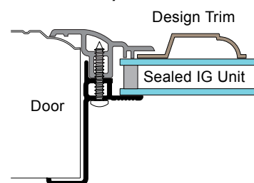
HRF- IG Style Window Frame
