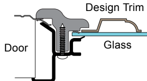
SWF- IP Style Window Frame
