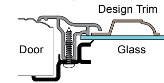
HWF- SG Style Window Frame
