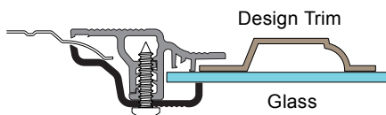
SRF- P Style Window Frame
