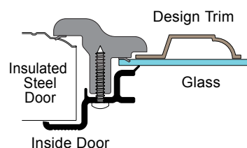
SWF- SG Style Window Frame
