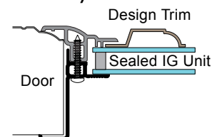
IMF- SG Style Window Frame
