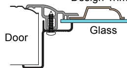
HRF- SG Style Window Frame Design Trim
