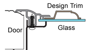
HRF- SG Style Window Frame
