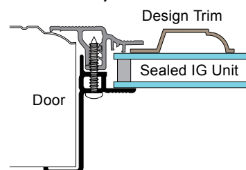
SRF- IG Style Window Frame
