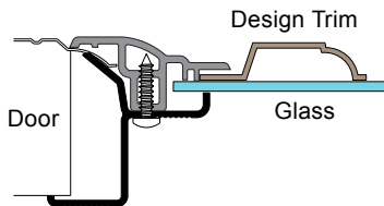
HRF- IP Style Window Frame
