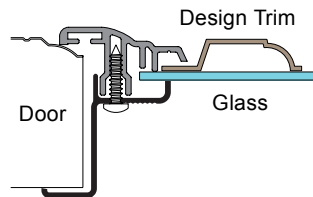
AWF-CLASSIC-SG Style Window Frame
