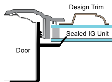
IMS- IG Style Window Frame
