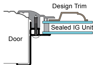
IMF- IG Style Window Frame
