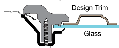
SWF- P Style Window Frame
