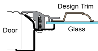
IMF- SG Style Window Frame
