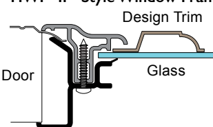
HWF- IP Style Window Frame
