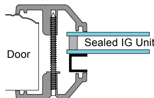
CMF- IG-SPACER Style Window Frame
