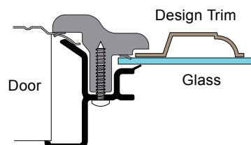
SWF-IP Style Window Frame
