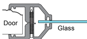
CMF- SG Style Window Frame
