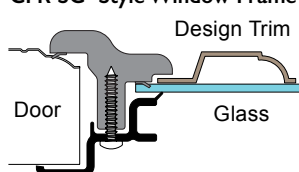
CFR-SG Style Window Frame
