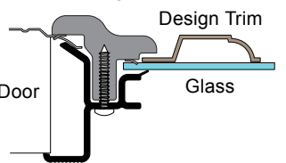
SWF- IP Style Window Frame
