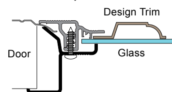
SRF- IP Style Window Frame
