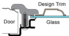
SWF- SG Style Window Frame
