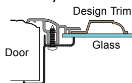
HRF- SG Style Window Frame
