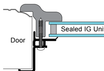
CWF- IG Style Window Frame
