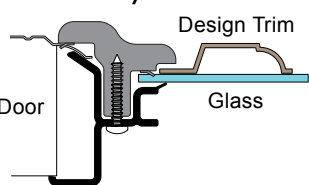
SWF- IP Style Window Frame
