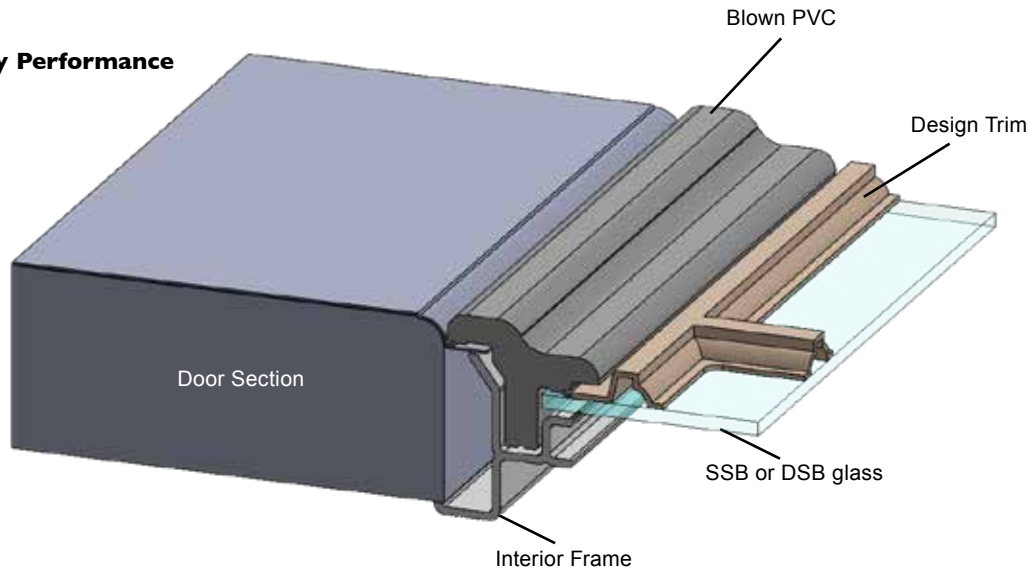
SWF-P Style Window Frame
