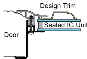
HRF- IG Style Window Frame
