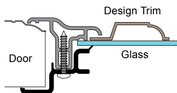
HWF- SG Style Window Frame
