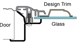
AWF-CLASSIC-IP Style Window Frame
