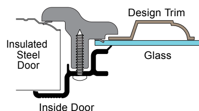
SWF- SG Style Window Frame
