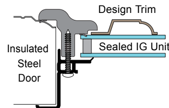
SWF- IG Style Window Frame
