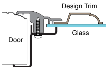
IMS- SG Style Window Frame
