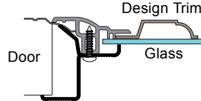
HRF- IP Style Window Frame
