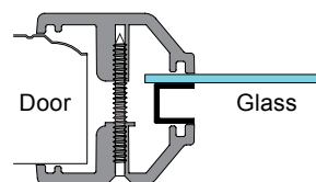
CMF- SG-SPACER Style Window Frame
