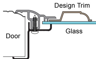
HRF- SG Style Window Frame
