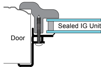
CWF- IG Style Window Frame
