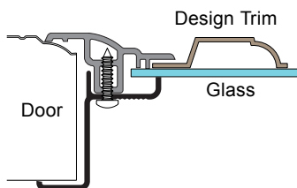
HRF- SG Style Window Frame
