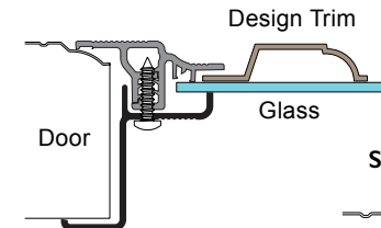
SRF- SG Style Window Frame
