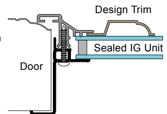
AWF-CONTEMPO-IG Style Window Frame
