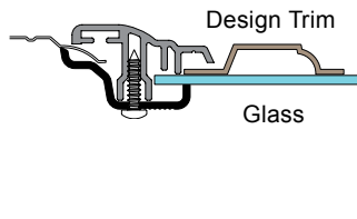
AWF-CLASSIC-P Style Window Frame
