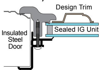
SWF- IG Style Window Frame
