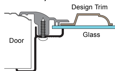
IMF- SG Style Window Frame
