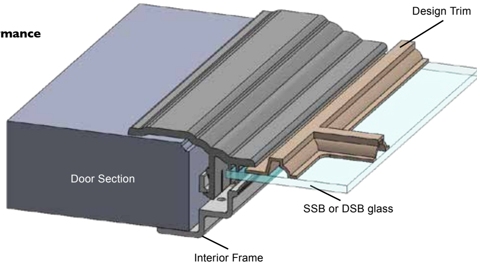
IMS- P Style Window Frame
