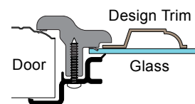
SWF- SG Style Window Frame
