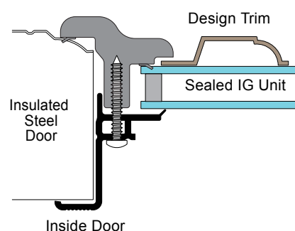
SWF- IG Style Window Frame
