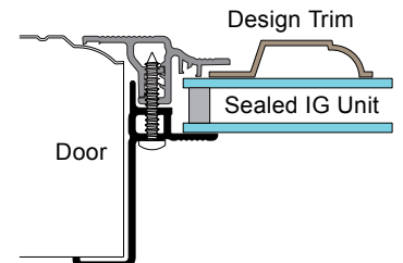
SRF- IG Style Window Frame
