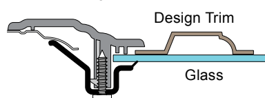
IMS- P Style Window Frame
