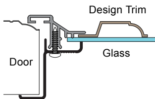
AWF-CONTEMPO-SG Style Window Frame
