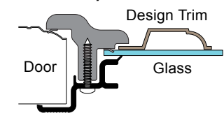
SWF- SG Style Window Frame
