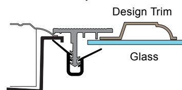
SPWF-PIF Style Window Frame
