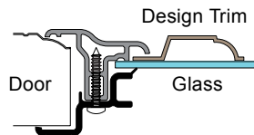
HWF- SG Style Window Frame
