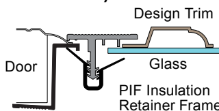
SPWF- PIF Style Window Frame
