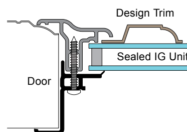
HWF- IG Style Window Frame
