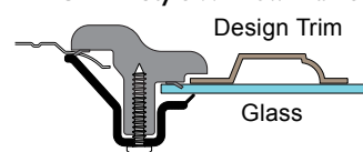
CFR-P Style Window Frame
