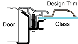
HWF- IP Style Window Frame
