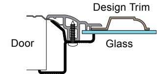
HRF- IP Style Window Frame
