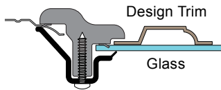
SWF-P Style Window Frame
