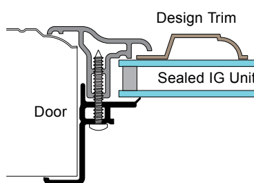
HWF- IG Style Window Frame
