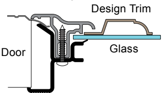
HWF- IP Style Window Frame
