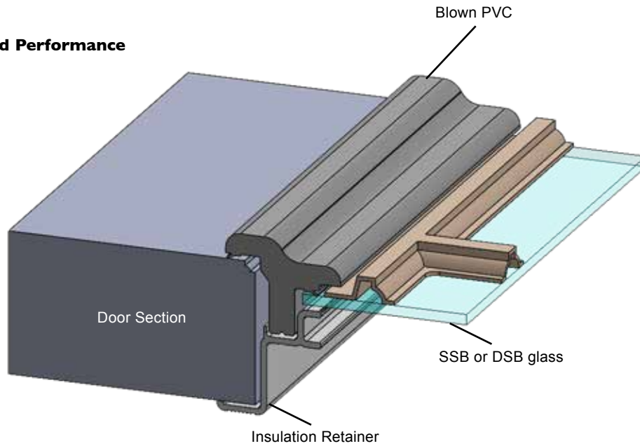
CWF- P Style Window Frame
