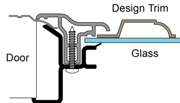
HWF- IP Style Window Frame
