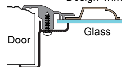
IMF- SG Style Window Frame Design Trim
