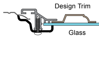
AWF-CONTEMPO-P Style Window Frame
