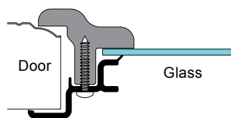
CWF- SG Style Window Frame
