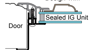
IMF- SG Style Window Frame Design Trim
