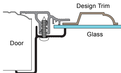
SRF- SG Style Window Frame
