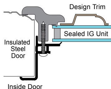
SWF- IG Style Window Frame
