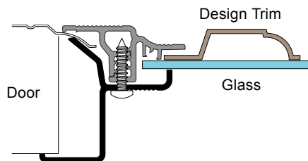
SRF- IP Style Window Frame
