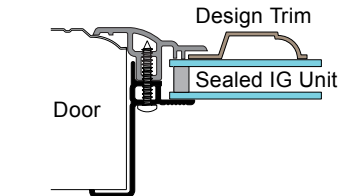
HRF- IG Style Window Frame
