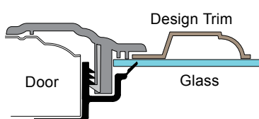
IMS- SG Style Window Frame
