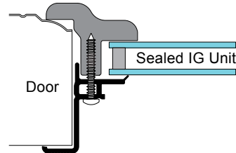
CWF- IG Style Window Frame
