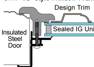
SWF- IG Style Window Frame
