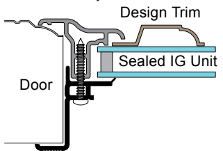
HWF- IG Style Window Frame
