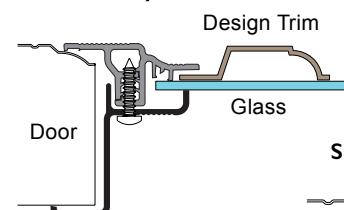
SRF- SG Style Window Frame
