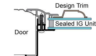
HRF- IG Style Window Frame
