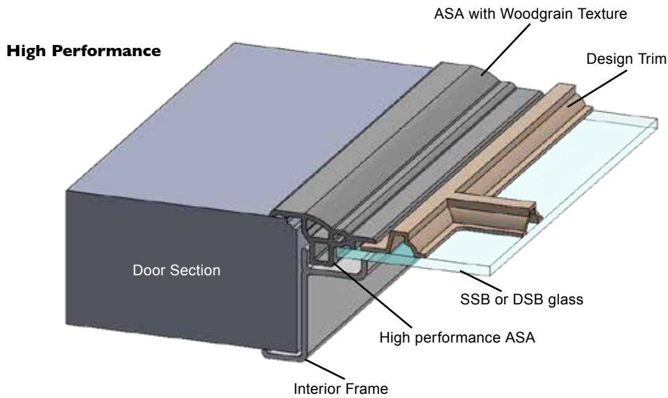
HRF- P Style Window Frame
