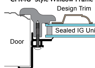
CFR-IG Style Window Frame
