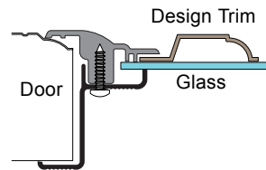
IMF- IP Style Window Frame
